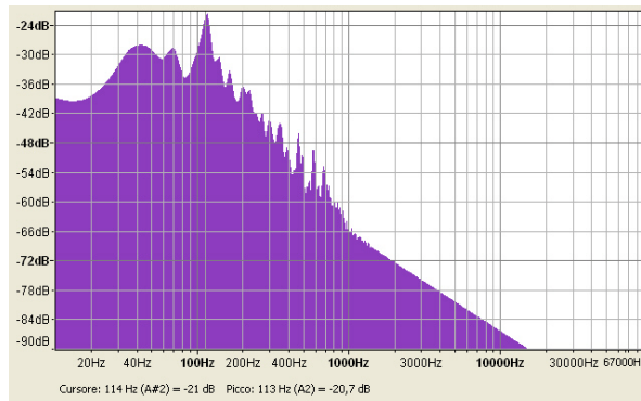
Figure 8 – The typical aspect of resonance at 114Hz found in Hal Saflieni Hypogeum in Malta. The resonance was stimulated by a sciamanic drum, but if the drum were drummed by soft hand instead of by a ram there were no resonance by the environment (Debertolis et al. 2015).
